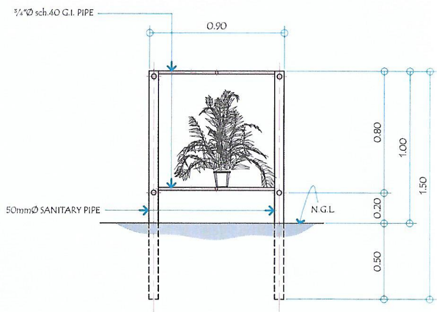
TYPICAL END ELEVATION SCALE: 1 : 25m
