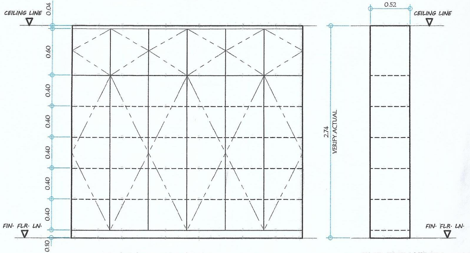
FRONT ELEVATION (CABINET-1) SCALE: 1:30 M
