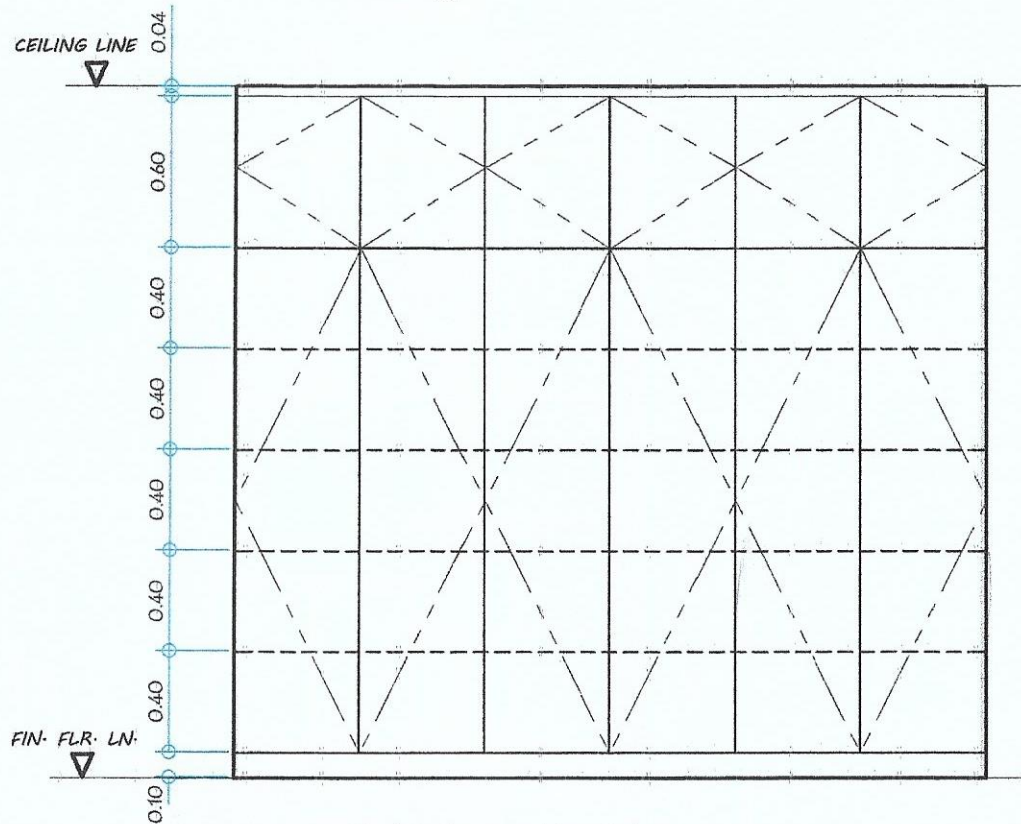
FRONT ELEVATION (CABINET-1) SCALE: 1:30 M
