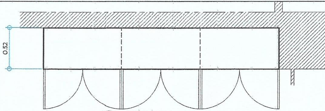
TOP VIEW (CABINET-1) SCALE: 1:30 M
