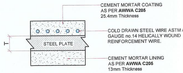
DETAIL DRAWING
