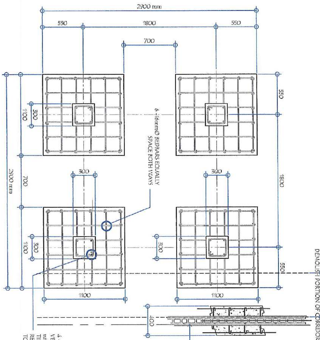
FOUNDATION PLAN SCALE: 1:30 M
