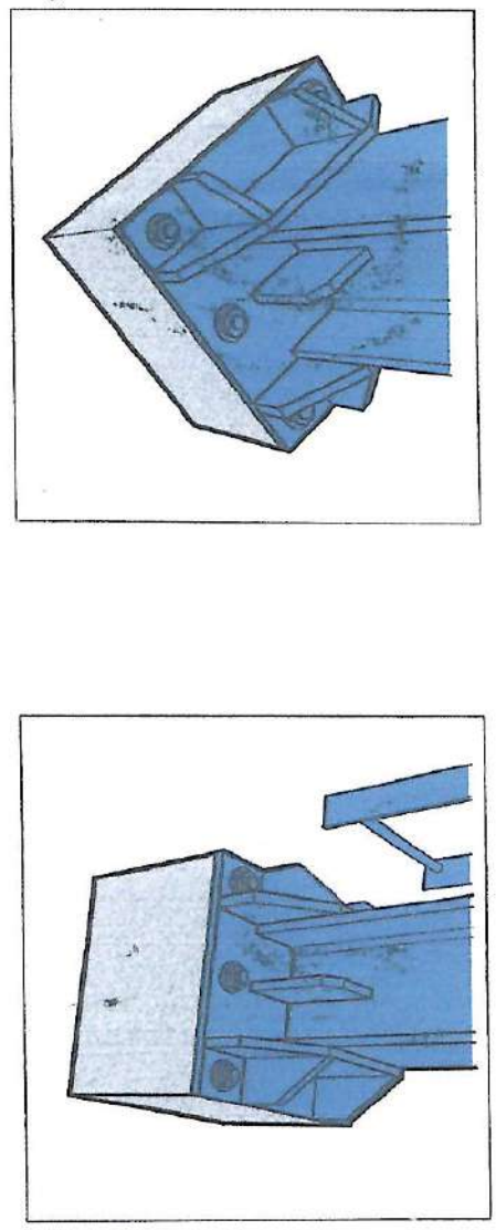
PERSPECTIVE (BASE PLATE)
