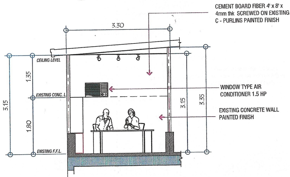
FRONT CROSS-SECTION SCALE: 14 : 1 M
