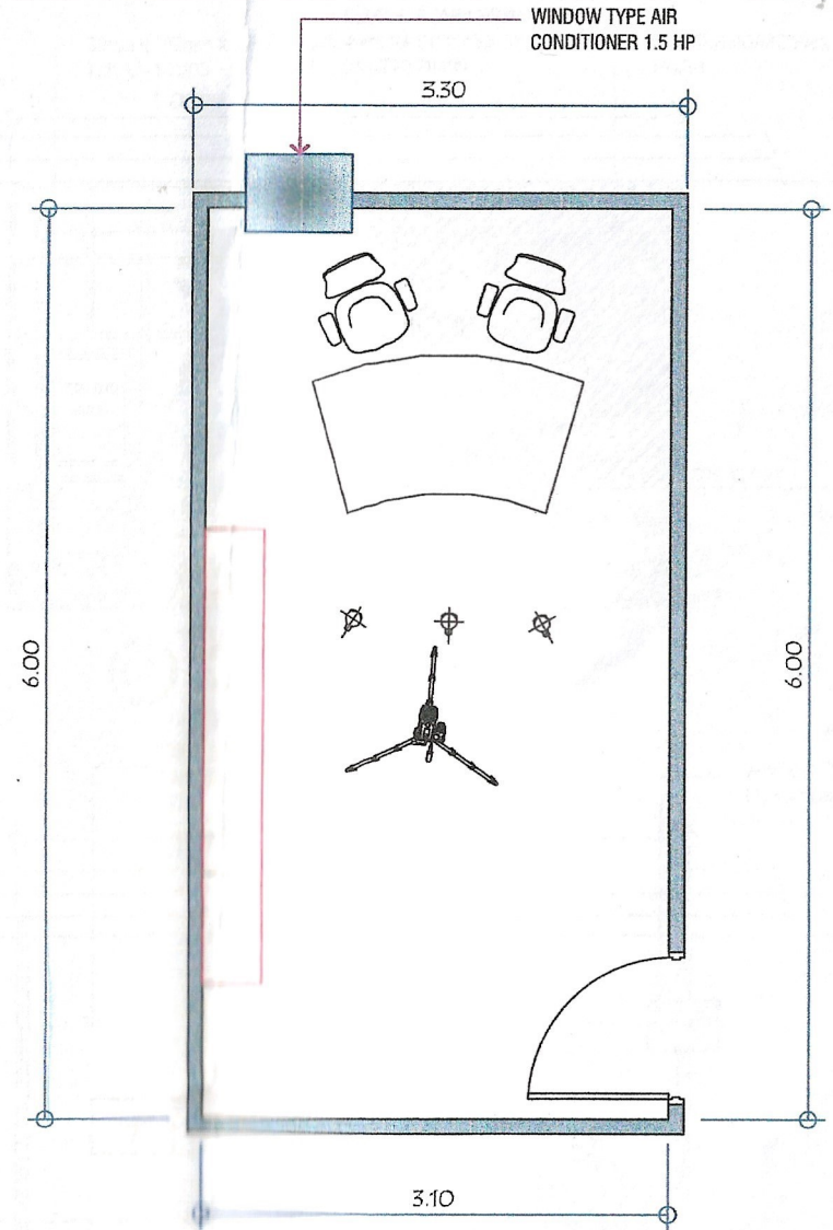
PROPOSED FLOOR PLAN SCALE: 20:1 M
