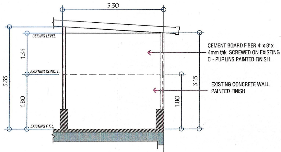
REAR CROSS-SECTION SCALE: 14 : 1 M
