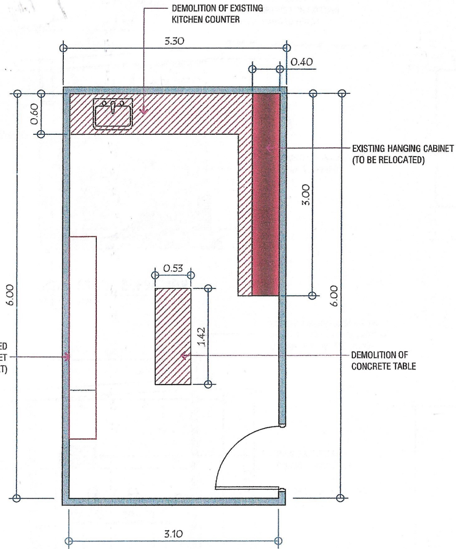
EXISTING FLOOR PLAN SCALE: 20:1 M
