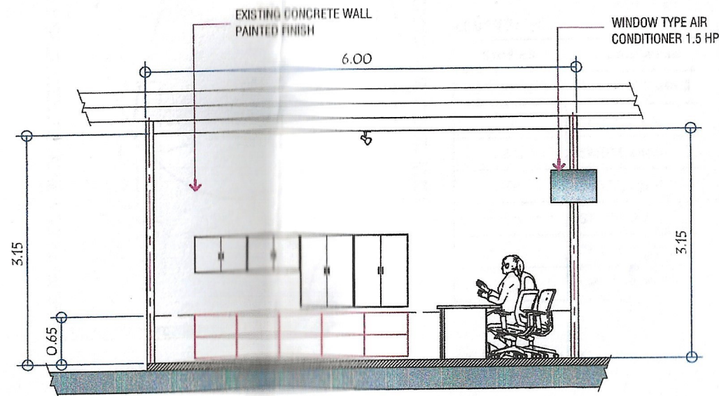
RIGHT SIDE CROSS-SECTION SCALE: 14 : 1 M
