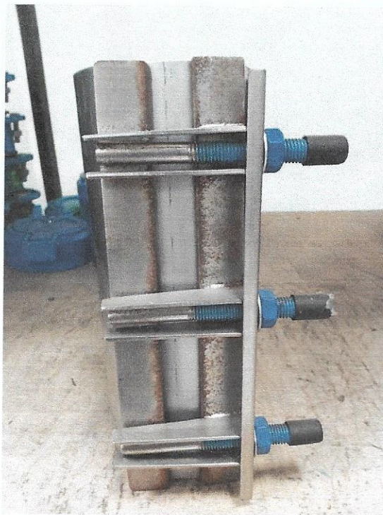
REPAIR CLAMP100mm
