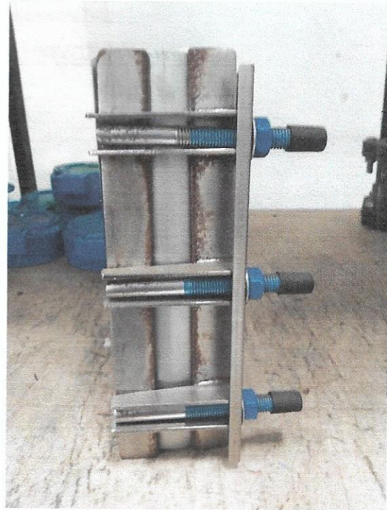
REPAIR CLAMP 75mm
