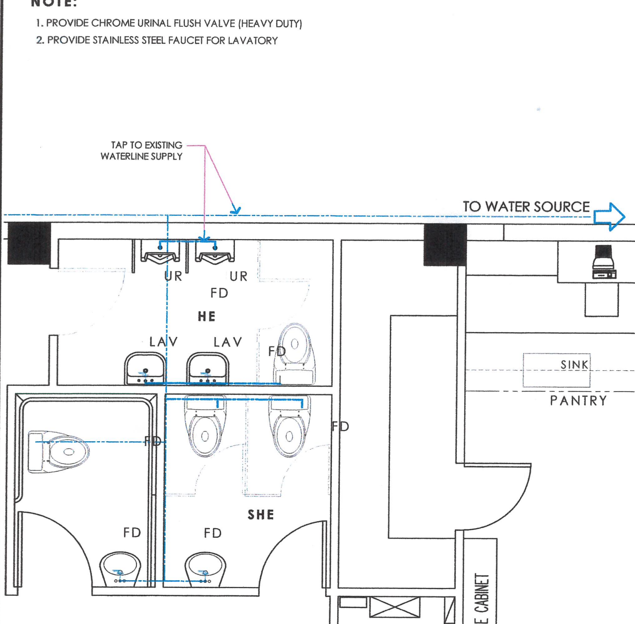
01 P 02 FLOOR PLAN (WATERLINE LAYOUT) SCALE : NTS
