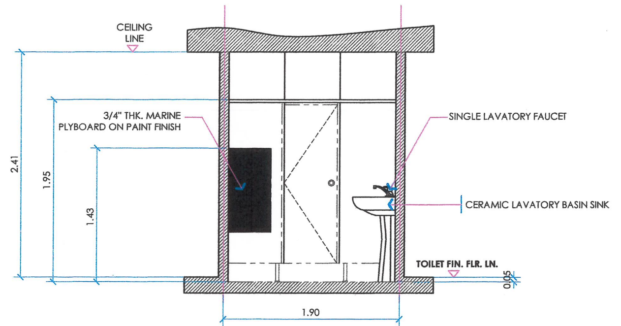
03 A-02 DETAIL SECTION (MEN'S TOILET) SCALE : 1:40
