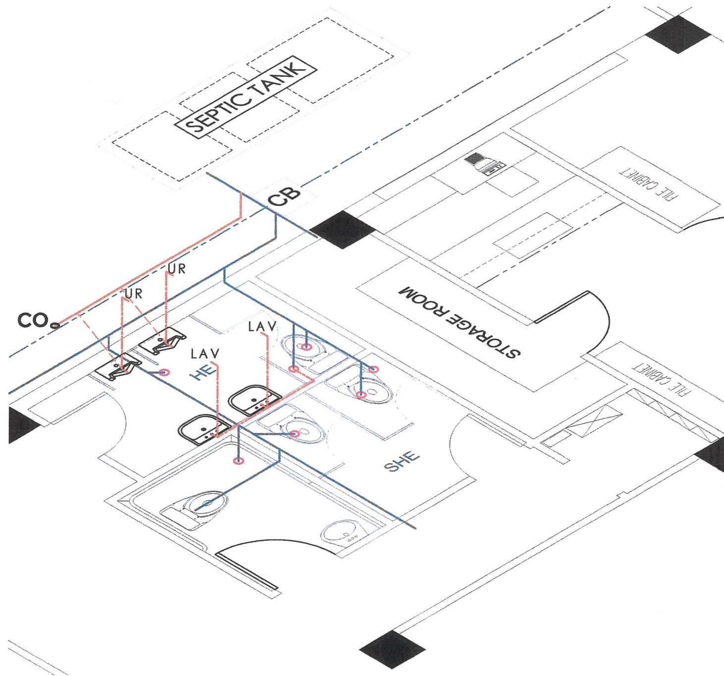
02 ISOMETRIC DIAGRAM (SEWER & DRAINAGE LAYOUT) SCALE : NTS
