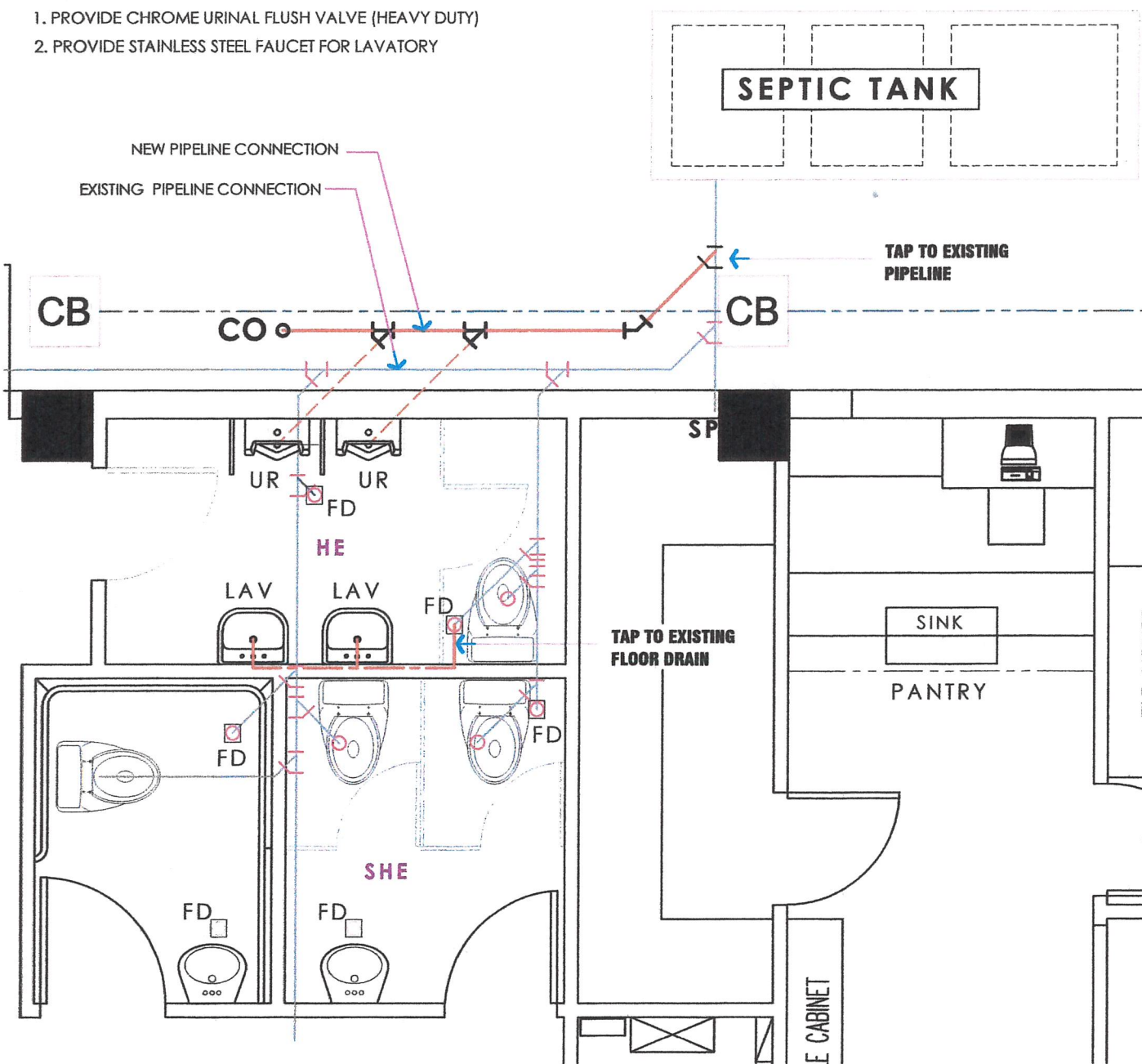
01 FLOOR PLAN (SEWER & DRAINAGE LAYOUT) SCALE : NTS
