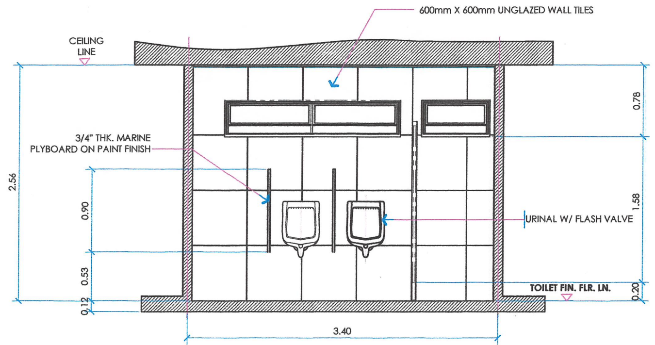
02 A-02 DETAIL SECTION (MEN'S TOILET) SCALE : 1:40
