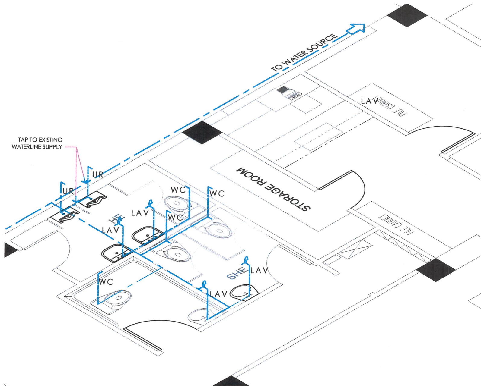
02 P 02 ISOMETRIC DIAGRAM (WATERLINE LAYOUT) SCALE : NTS
