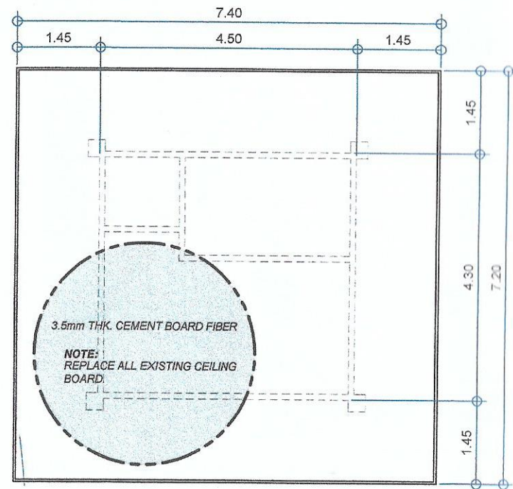
CEILING PLAN SCALE: NTS
