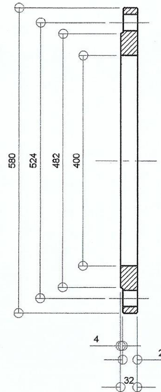
SECTION
