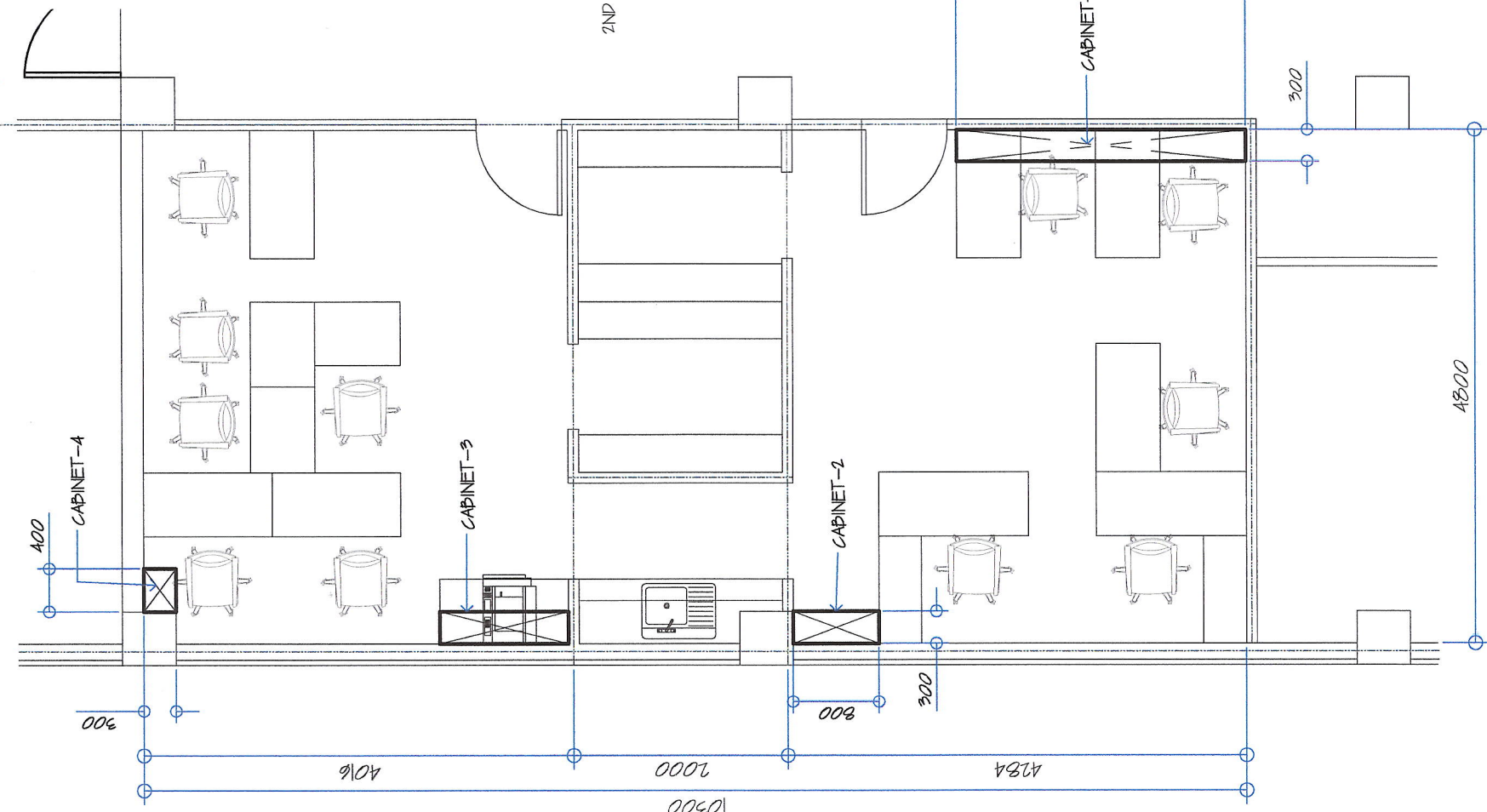
01 FLOOR PLAN B-02 SCALE: 1 : 60 M
