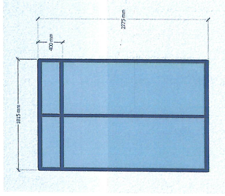
ALUMINUM AND GLASS PARTITION - 6MM CLEAR GLASS SCALE: NOT TO SCALE
